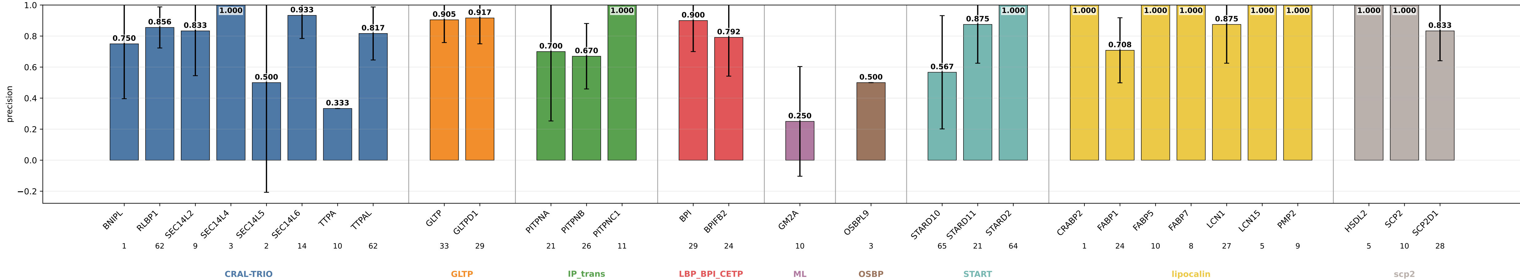
ge_s15_prothid32_hid64_noreg_liptail precision by subgroup ge_s15_prothid32_hid64_noreg_liptail | class weights | lr=0.0001 | weight_decay=1e-05 | final_m=4 | final_dropout=0.0 | hiddim=64 | heads=8 | batch=16 | ep=120 | seeds=0,1,2,3,4
