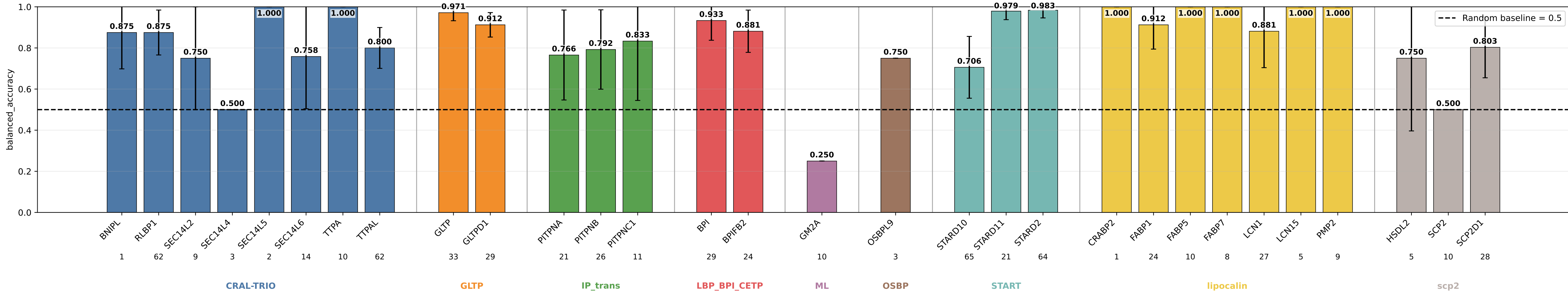
ge_s15_prothid32_hid64_noreg_lr3e5 balanced_accuracy by subgroup ge_s15_prothid32_hid64_noreg_lr3e5 | class weights | lr=3e-05 | weight_decay=1e-05 | final_m=4 | final_dropout=0.0 | hiddim=64 | heads=8 | batch=16 | ep=120 | seeds=0,1,2,3,4
