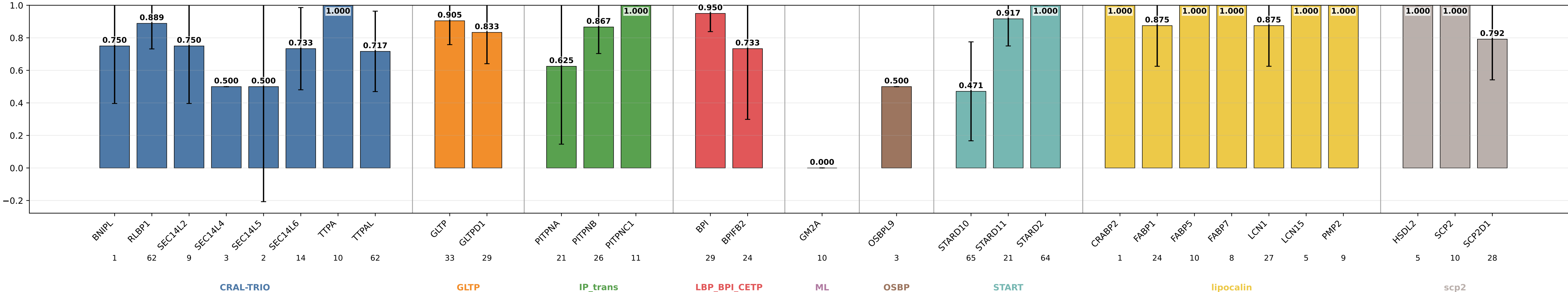
ge_s15_prothid32_hid64_noreg_lr3e5 precision by subgroup ge_s15_prothid32_hid64_noreg_lr3e5 | class weights | lr=3e-05 | weight_decay=1e-05 | final_m=4 | final_dropout=0.0 | hiddim=64 | heads=8 | batch=16 | ep=120 | seeds=0,1,2,3,4
