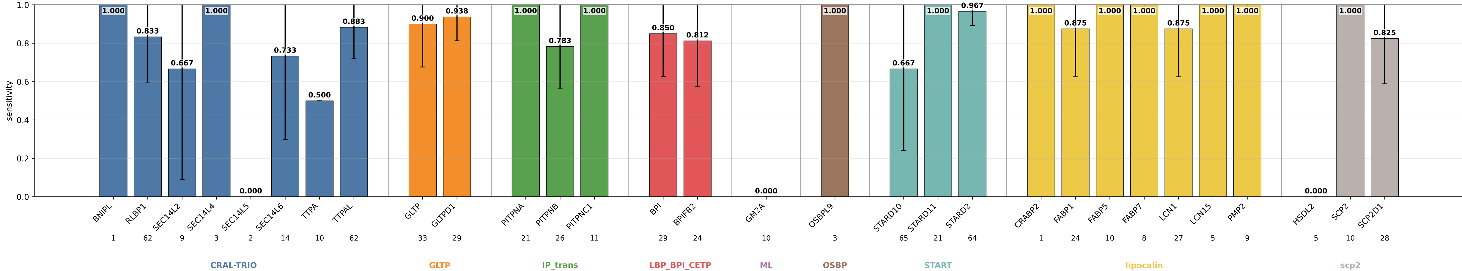
ge_s15_prothid32_hid64_noreg_m8 sensitivity by subgroup ge_s15_prothid32_hid64_noreg_m8 | class weights | lr=0.0001 | weight_decay=1e-05 | final_m=8 | final_dropout=0.0 | hiddim=64 | heads=8 | batch=16 | ep=120 | seeds=0,1,2,3,4
