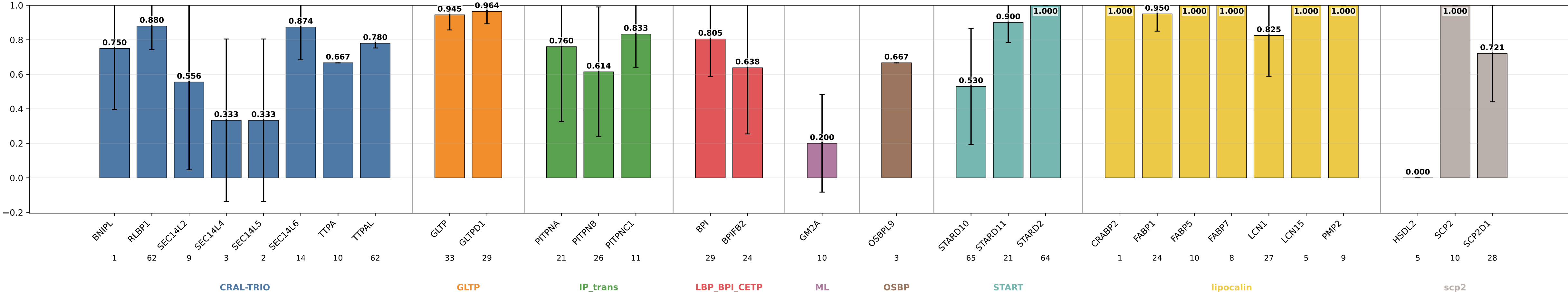
ge_s15_prothid32_hid64_noreg_nodebilin F1 by subgroup ge_s15_prothid32_hid64_noreg_nodebilin | class weights | lr=0.0001 | weight_decay=1e-05 | final_m=4 | final_dropout=0.0 | hiddim=64 | heads=8 | batch=16 | ep=120 | seeds=0,1,2,3,4
