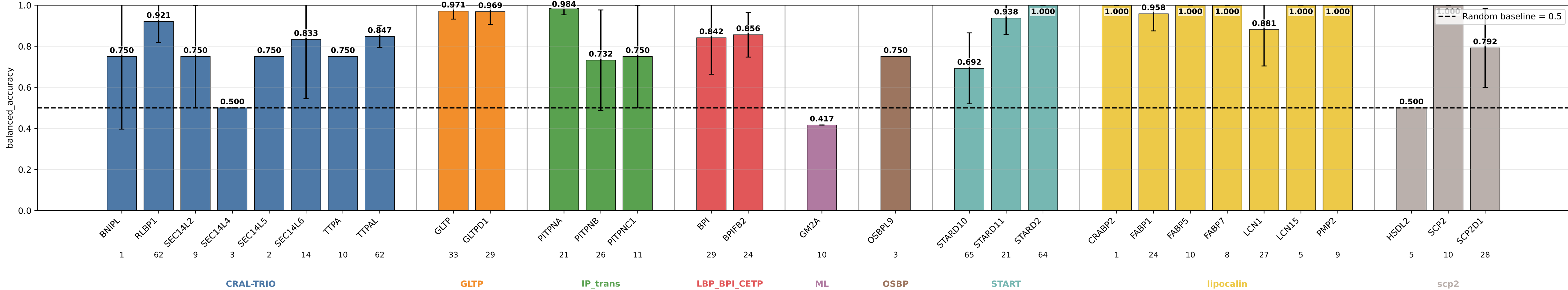
ge_s15_prothid32_hid64_noreg_nodebilin balanced_accuracy by subgroup ge_s15_prothid32_hid64_noreg_nodebilin | class weights | lr=0.0001 | weight_decay=1e-05 | final_m=4 | final_dropout=0.0 | hiddim=64 | heads=8 | batch=16 | ep=120 | seeds=0,1,2,3,4
