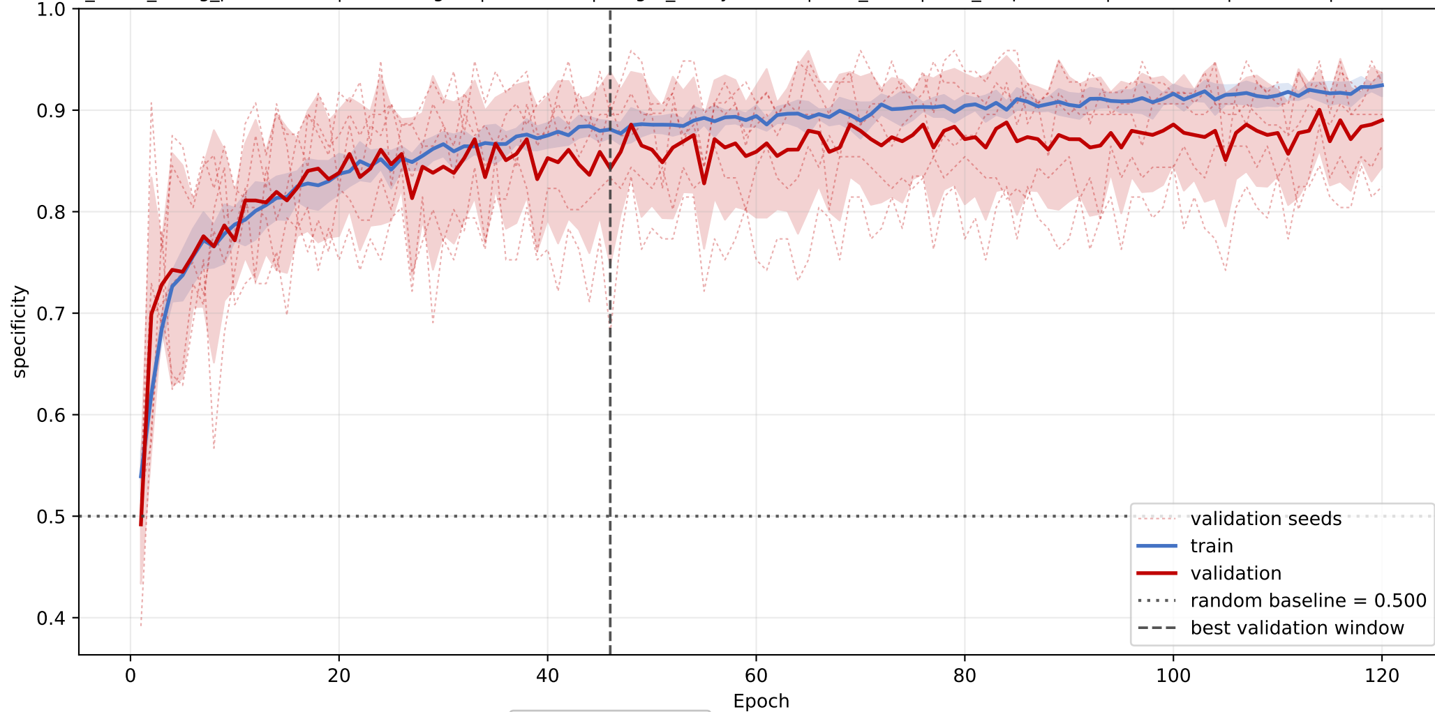
species15: mean specificity learning curve across seeds
