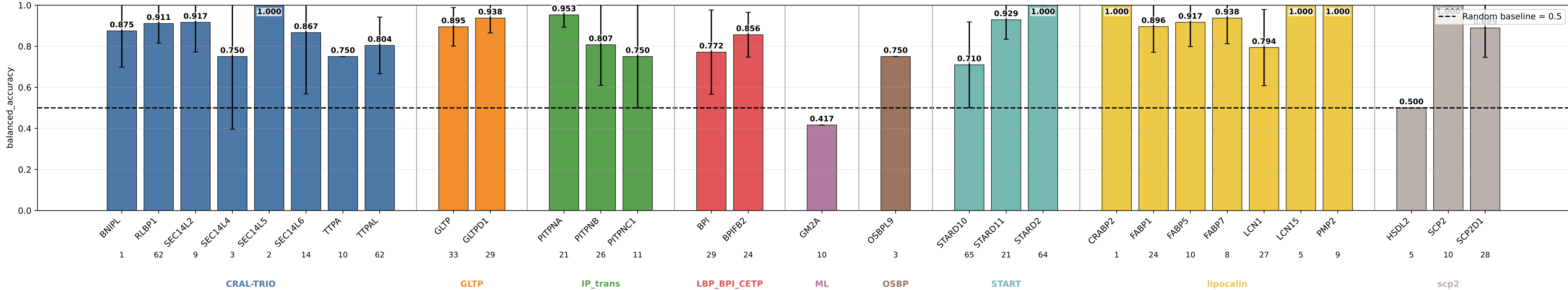
ge_s15_prothid32_noreg balanced_accuracy by subgroup ge_s15_prothid32_noreg | class weights | lr=0.0001 | weight_decay=1e-05 | final_m=4 | final_dropout=0.0 | hiddim=8 | heads=8 | batch=16 | ep=120 | seeds=0,1,2,3,4
