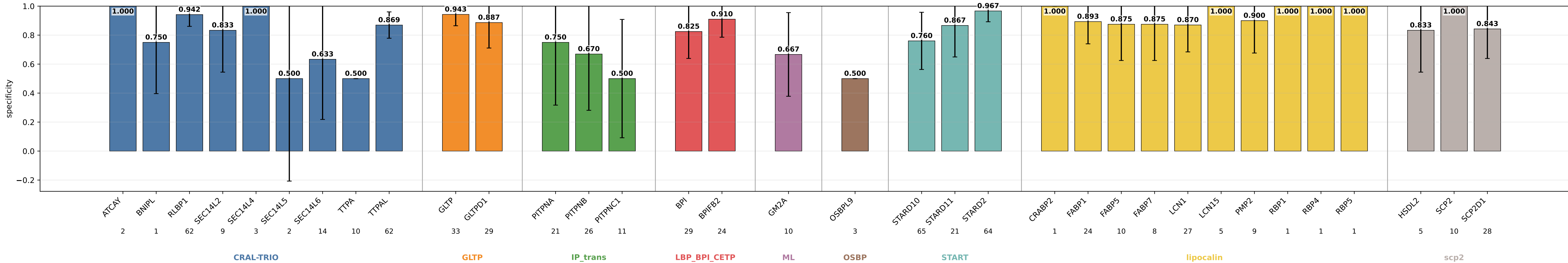
ge_s15_prothid32_wd1e5 specificity by subgroup ge_s15_prothid32_wd1e5 | class weights | lr=0.0001 | weight_decay=1e-05 | final_m=4 | final_dropout=0.1 | hiddim=8 | heads=8 | batch=16 | ep=120 | seeds=0,1,2,3,4
