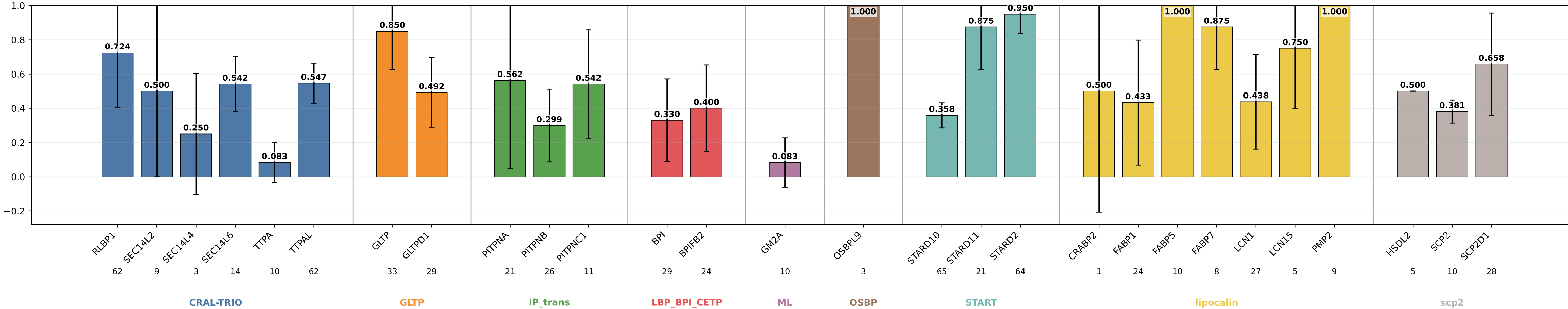
mlp_s15_mbw_hid16 precision by subgroup mlp_s15_mbw_hid16 | class weights | lr=0.0001 | weight_decay=0.01 | final_m=4 | final_dropout=0.1 | hiddim=16 | heads=8 | batch=16 | ep=120 | seeds=0,1,2,3,4
