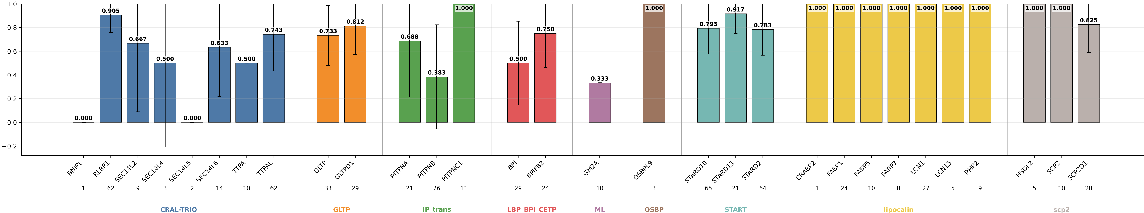
mlp_s15_mbw_hid16 sensitivity by subgroup mlp_s15_mbw_hid16 | class weights | lr=0.0001 | weight_decay=0.01 | final_m=4 | final_dropout=0.1 | hiddim=16 | heads=8 | batch=16 | ep=120 | seeds=0,1,2,3,4
