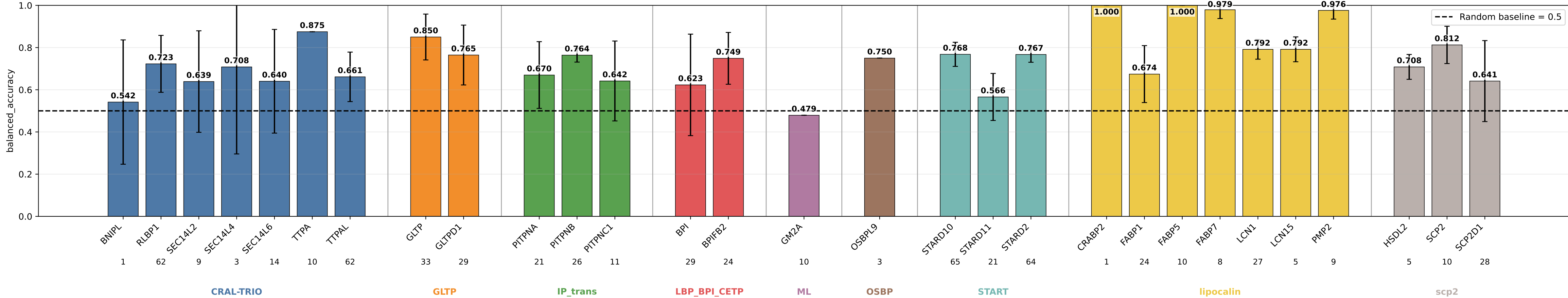
mlp_s15_mbw_hid32_d11 balanced_accuracy by subgroup mlp_s15_mbw_hid32_d11 | class weights | lr=0.0001 | weight_decay=0.01 | final_m=4 | final_dropout=0.1 | hiddim=32 | heads=8 | batch=16 | ep=120 | seeds=0,1,2,3,4
