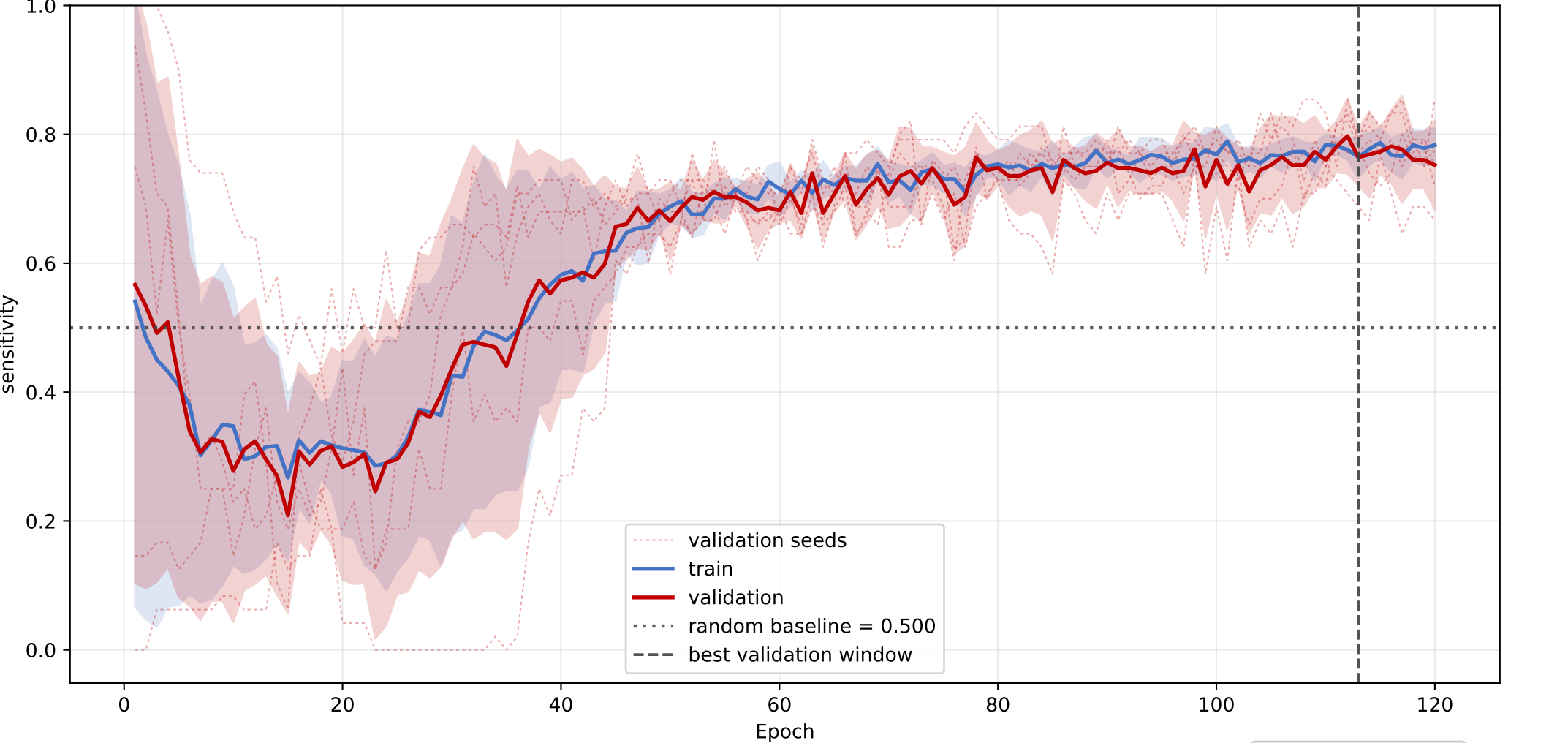
species15: mean sensitivity learning curve across seeds
