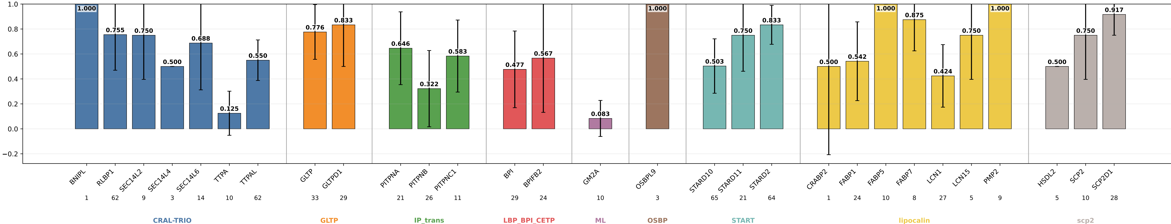
mlp_s15_mbw_hid32_dpt0 precision by subgroup mlp_s15_mbw_hid32_dpt0 | class weights | lr=0.0001 | weight_decay=0.01 | final_m=4 | final_dropout=0.0 | hiddim=32 | heads=8 | batch=16 | ep=120 | seeds=0,1,2,3,4
