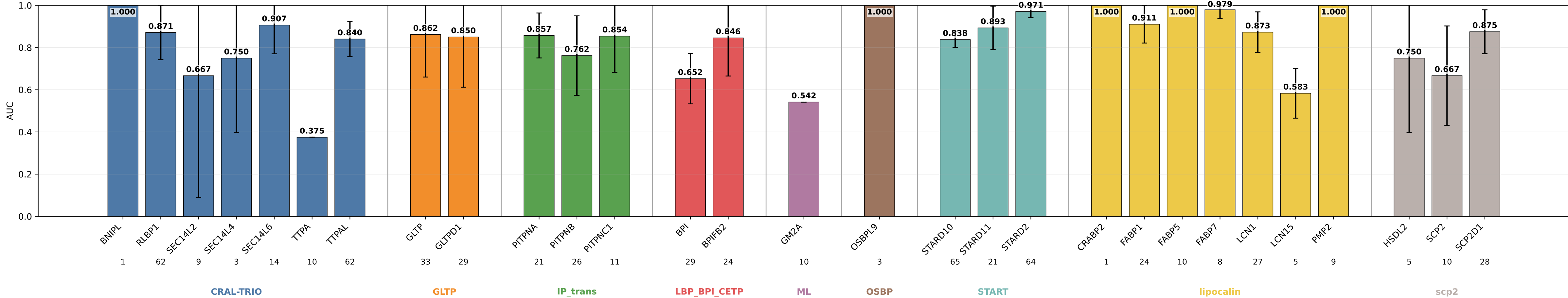
mlp_s15_mbw_lipprop AUC by subgroup mlp_s15_mbw_lipprop | class weights | lr=0.0001 | weight_decay=0.01 | final_m=4 | final_dropout=0.1 | hiddim=8 | heads=8 | batch=16 | ep=120 | seeds=0,1,2,3,4
