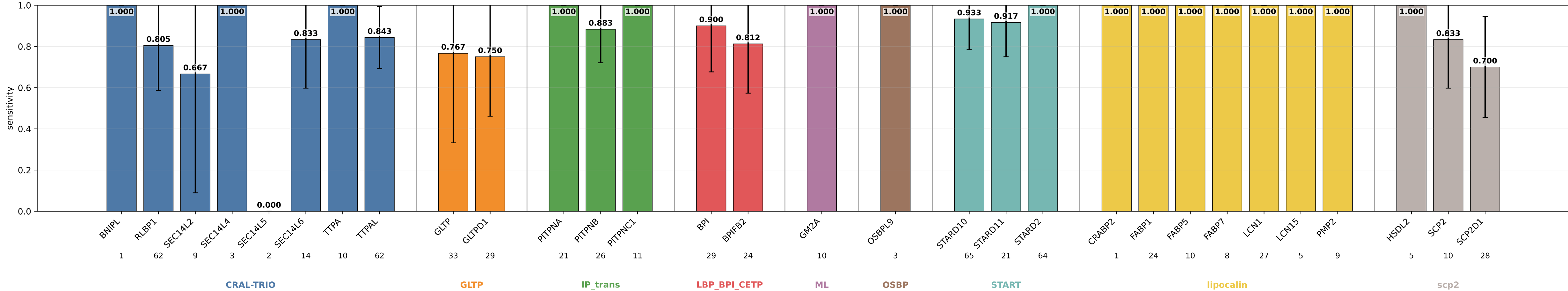
mlp_s15_nomb_hid128 sensitivity by subgroup mlp_s15_nomb_hid128 | class weights | lr=0.0001 | weight_decay=0.01 | final_m=4 | final_dropout=0.1 | hiddim=128 | heads=8 | batch=16 | ep=120 | seeds=0,1,2,3,4
