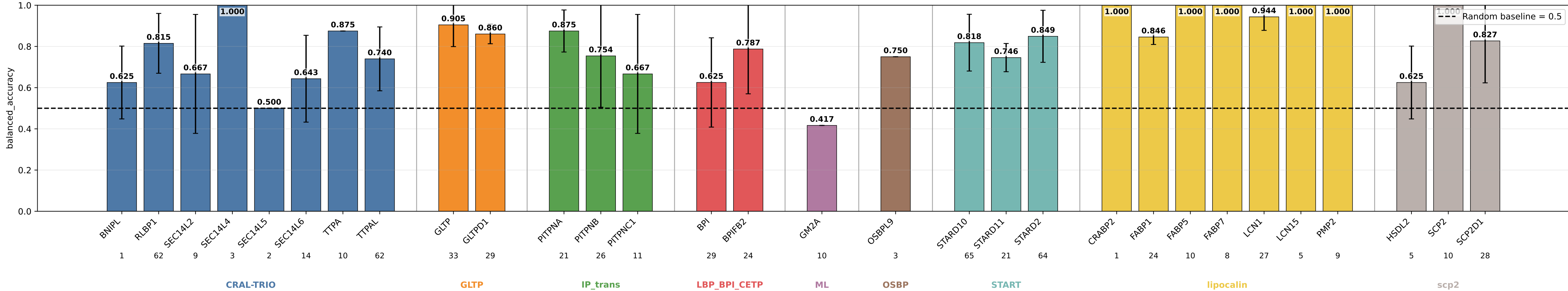
mlp_s15_nomb_hid32_m8_d11 balanced_accuracy by subgroup mlp_s15_nomb_hid32_m8_d11 | class weights | lr=0.0001 | weight_decay=0.01 | final_m=4 | final_dropout=0.1 | hiddim=32 | heads=8 | batch=16 | ep=120 | seeds=0,1,2,3,4
