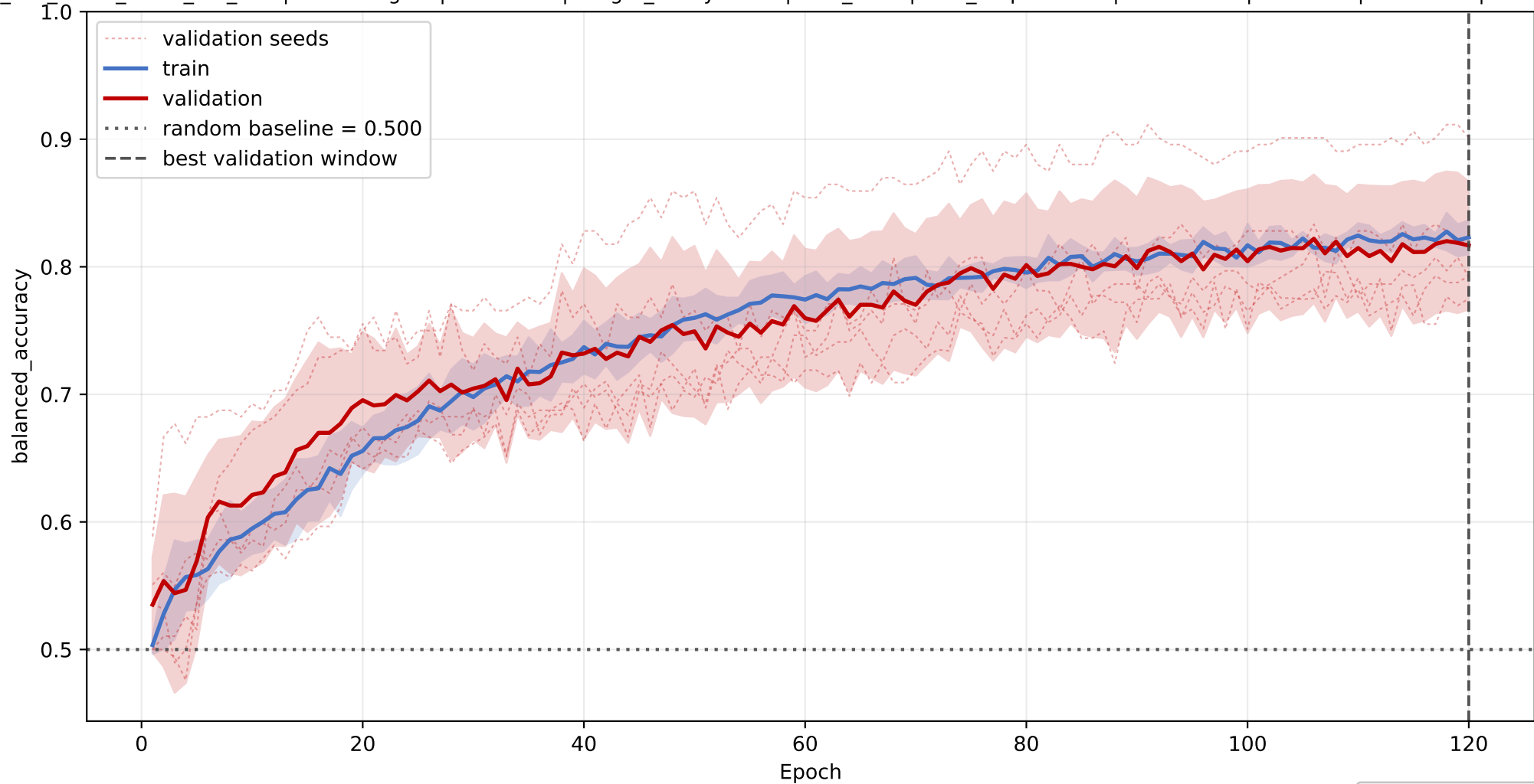
species15: mean balanced_accuracy learning curve across seeds
