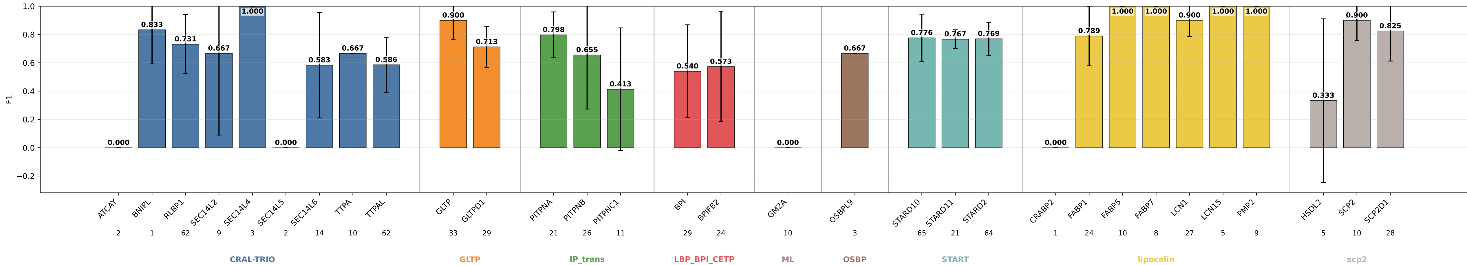
mlp_s15_nomb_hid32_m8_d12 F1 by subgroup mlp_s15_nomb_hid32_m8_d12 | class weights | lr=0.0001 | weight_decay=0.01 | final_m=4 | final_dropout=0.1 | hiddim=32 | heads=8 | batch=16 | ep=120 | seeds=0,1,2,3,4
