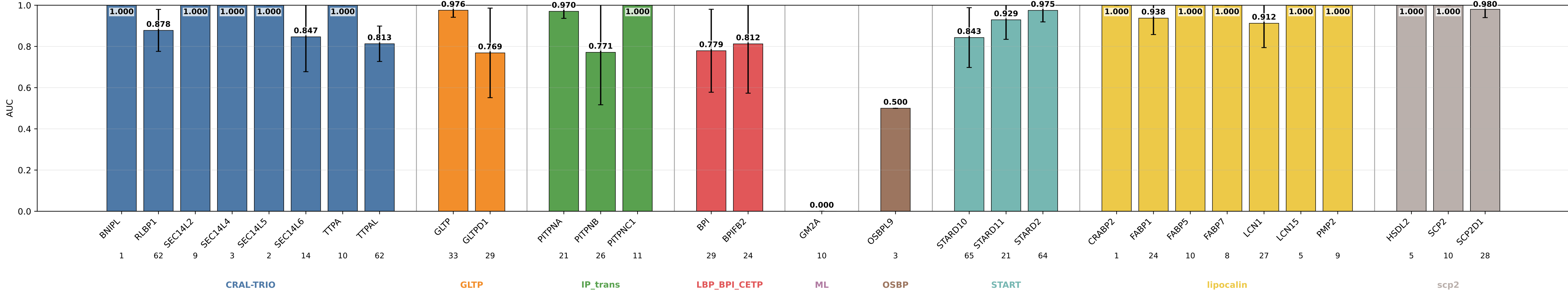
mlp_s15_nomb_hid32_m8_d14 AUC by subgroup mlp_s15_nomb_hid32_m8_d14 | class weights | lr=0.0001 | weight_decay=0.01 | final_m=4 | final_dropout=0.1 | hiddim=32 | heads=8 | batch=16 | ep=120 | seeds=0,1,2,3,4
