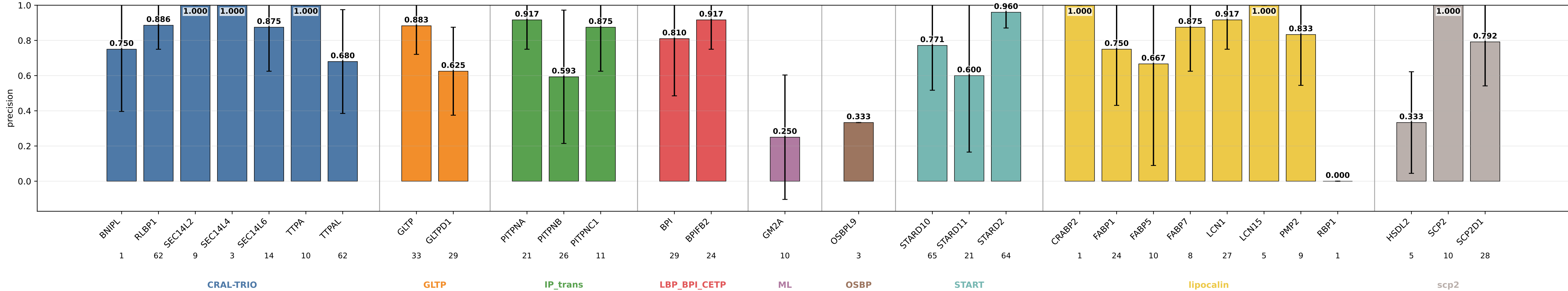
mlp_s15_nomb_hid64_3mlp precision by subgroup mlp_s15_nomb_hid64_3mlp | class weights | lr=0.0001 | weight_decay=0.01 | final_m=4 | final_dropout=0.1 | hiddim=64 | heads=8 | batch=16 | ep=120 | seeds=0,1,2,3,4
