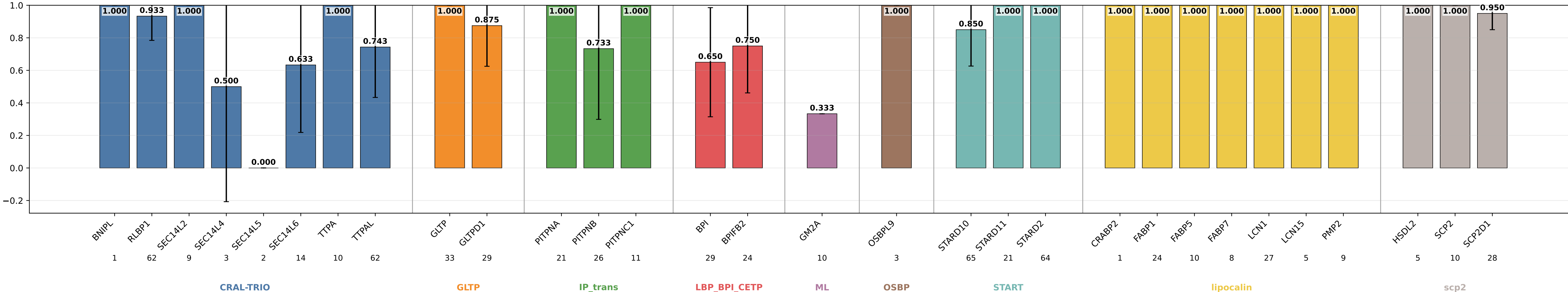
mlp_s15_nomb_hid64_3mlp sensitivity by subgroup mlp_s15_nomb_hid64_3mlp | class weights | lr=0.0001 | weight_decay=0.01 | final_m=4 | final_dropout=0.1 | hiddim=64 | heads=8 | batch=16 | ep=120 | seeds=0,1,2,3,4
