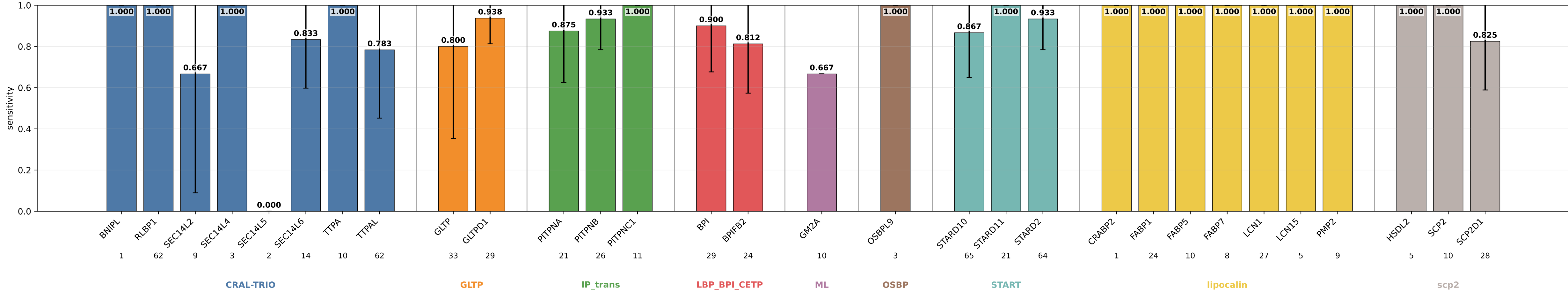
mlp_s15_nomb_hid64_ep360 sensitivity by subgroup mlp_s15_nomb_hid64_ep360 | class weights | lr=0.0001 | weight_decay=0.01 | final_m=4 | final_dropout=0.1 | hiddim=64 | heads=8 | batch=16 | ep=360 | seeds=0,1,2,3,4
