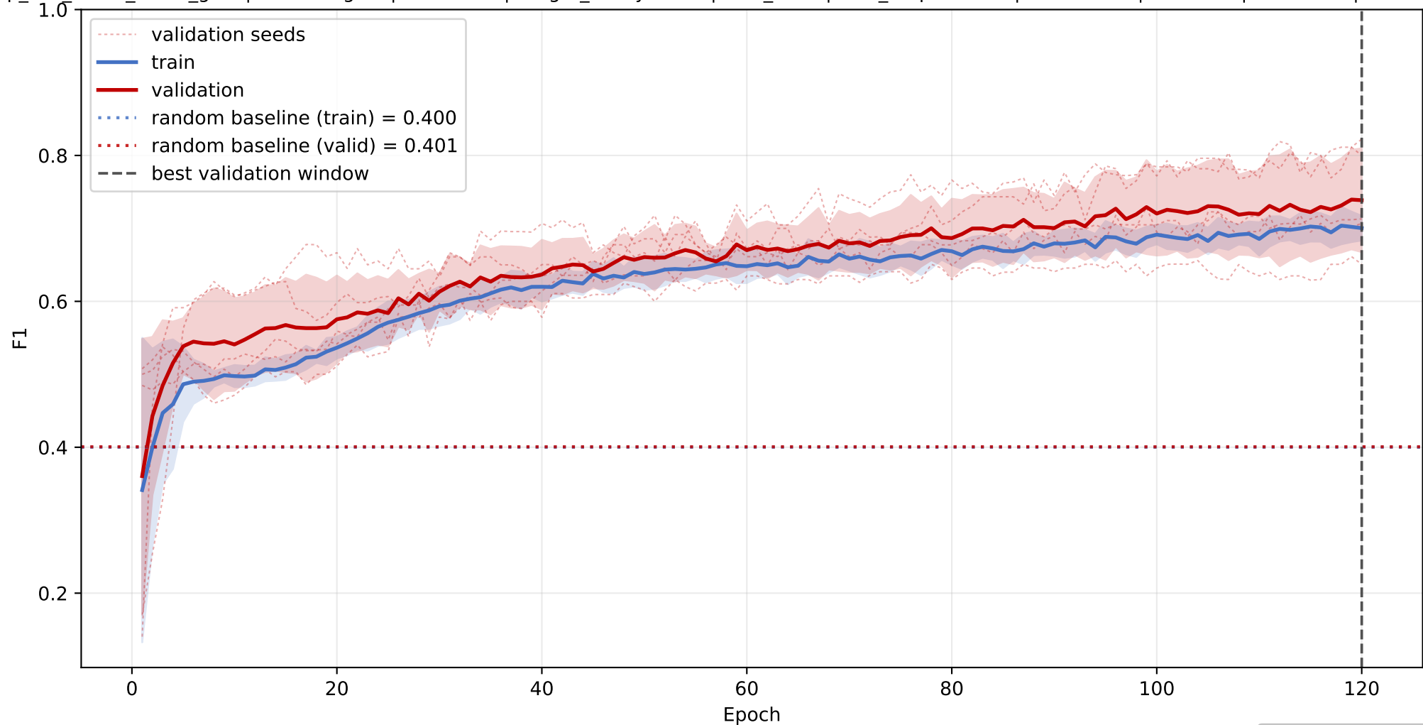
species15: mean F1 learning curve across seeds
