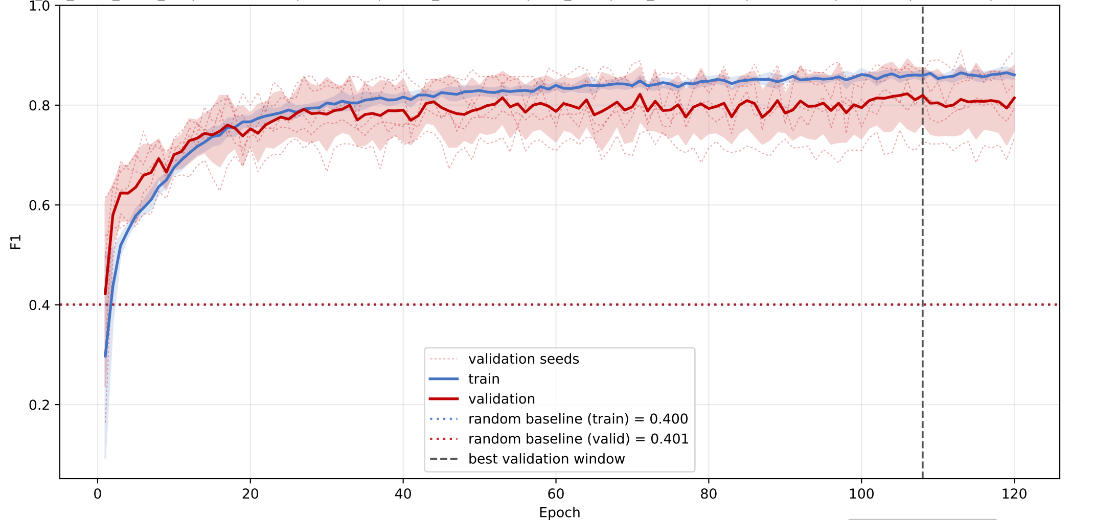
species15: mean F1 learning curve across seeds
