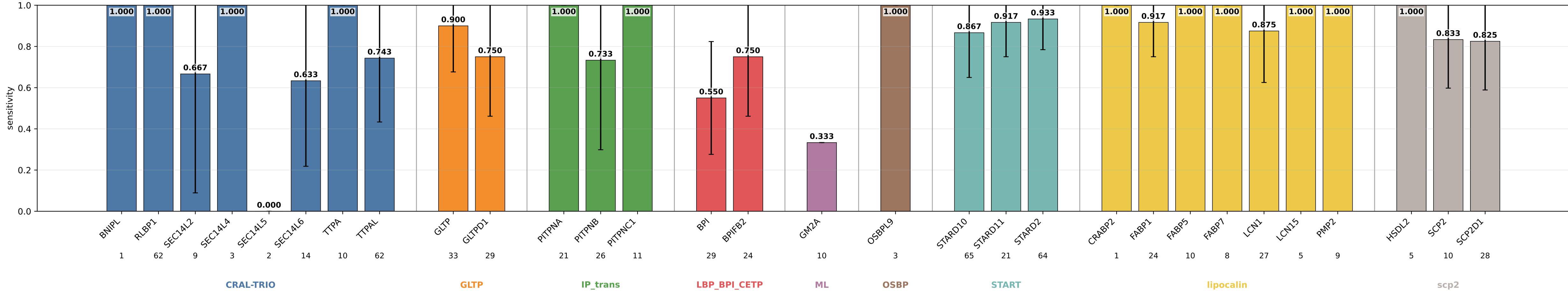
mlp_s15_nomb_hid64_m8_dpt0 sensitivity by subgroup mlp_s15_nomb_hid64_m8_dpt0 | class weights | lr=0.0001 | weight_decay=0.01 | final_m=4 | final_dropout=0.0 | hiddim=64 | heads=8 | batch=16 | ep=120 | seeds=0,1,2,3,4
