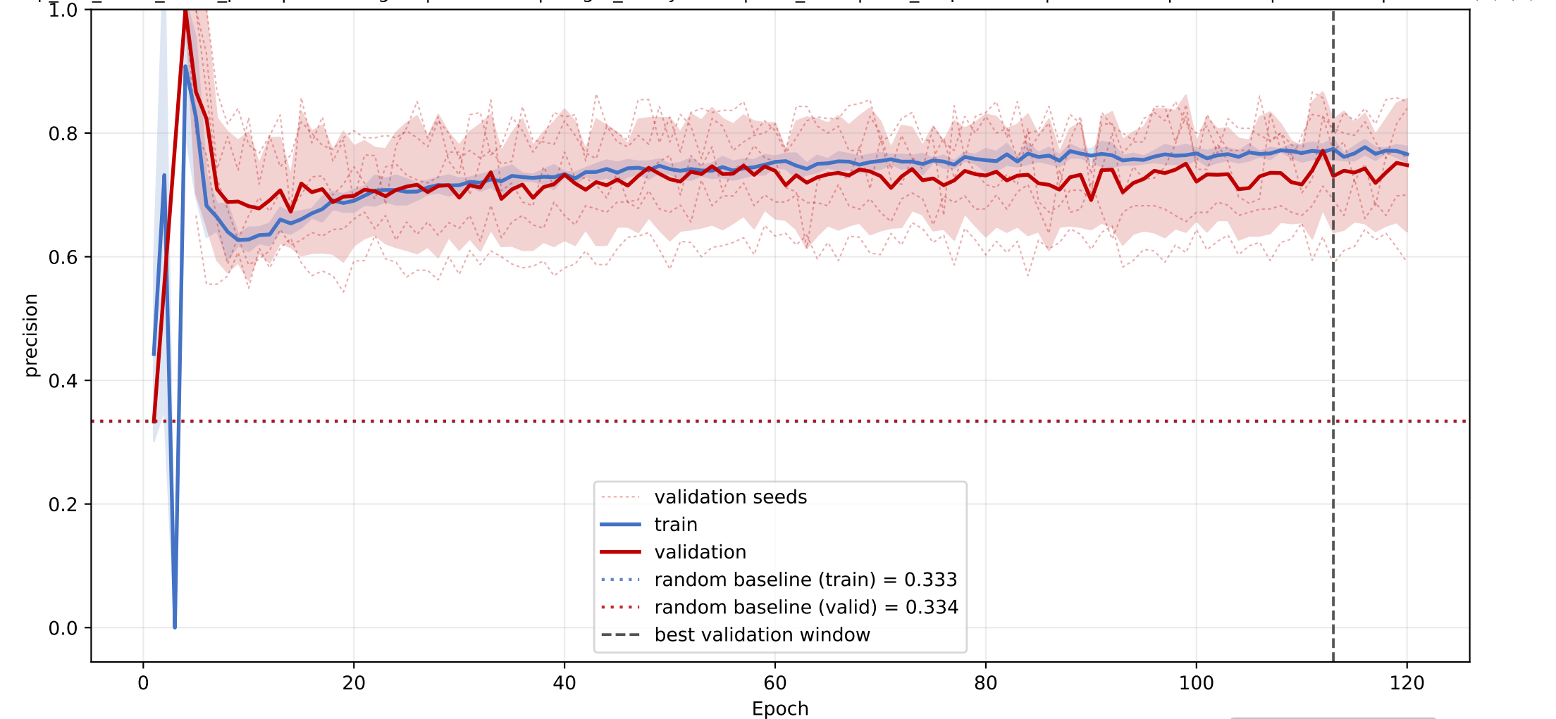
species15: mean precision learning curve across seeds
