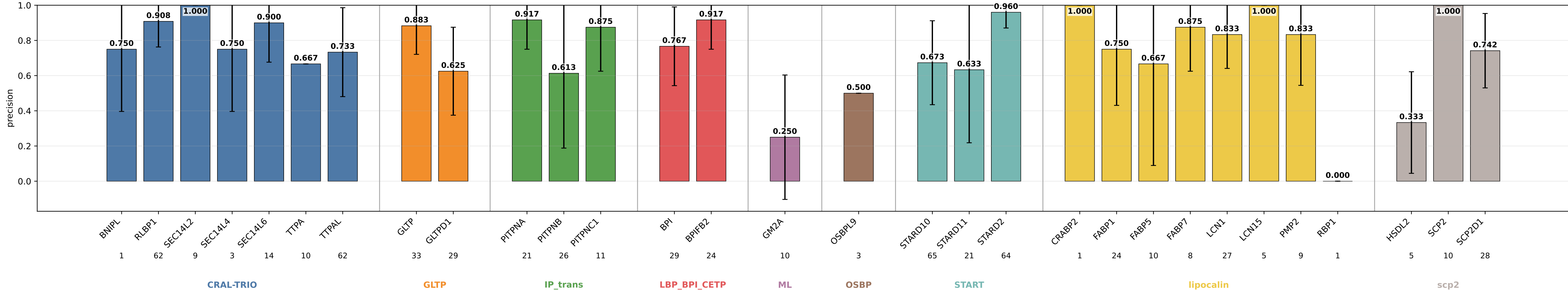
mlp_s15_nomb_hid64_relu precision by subgroup mlp_s15_nomb_hid64_relu | class weights | lr=0.0001 | weight_decay=0.01 | final_m=4 | final_dropout=0.1 | hiddim=64 | heads=8 | batch=16 | ep=120 | seeds=0,1,2,3,4
