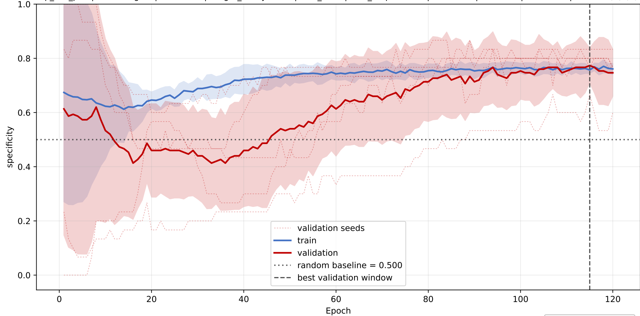
LPC+LPE+LPG: mean specificity learning curve across seeds
