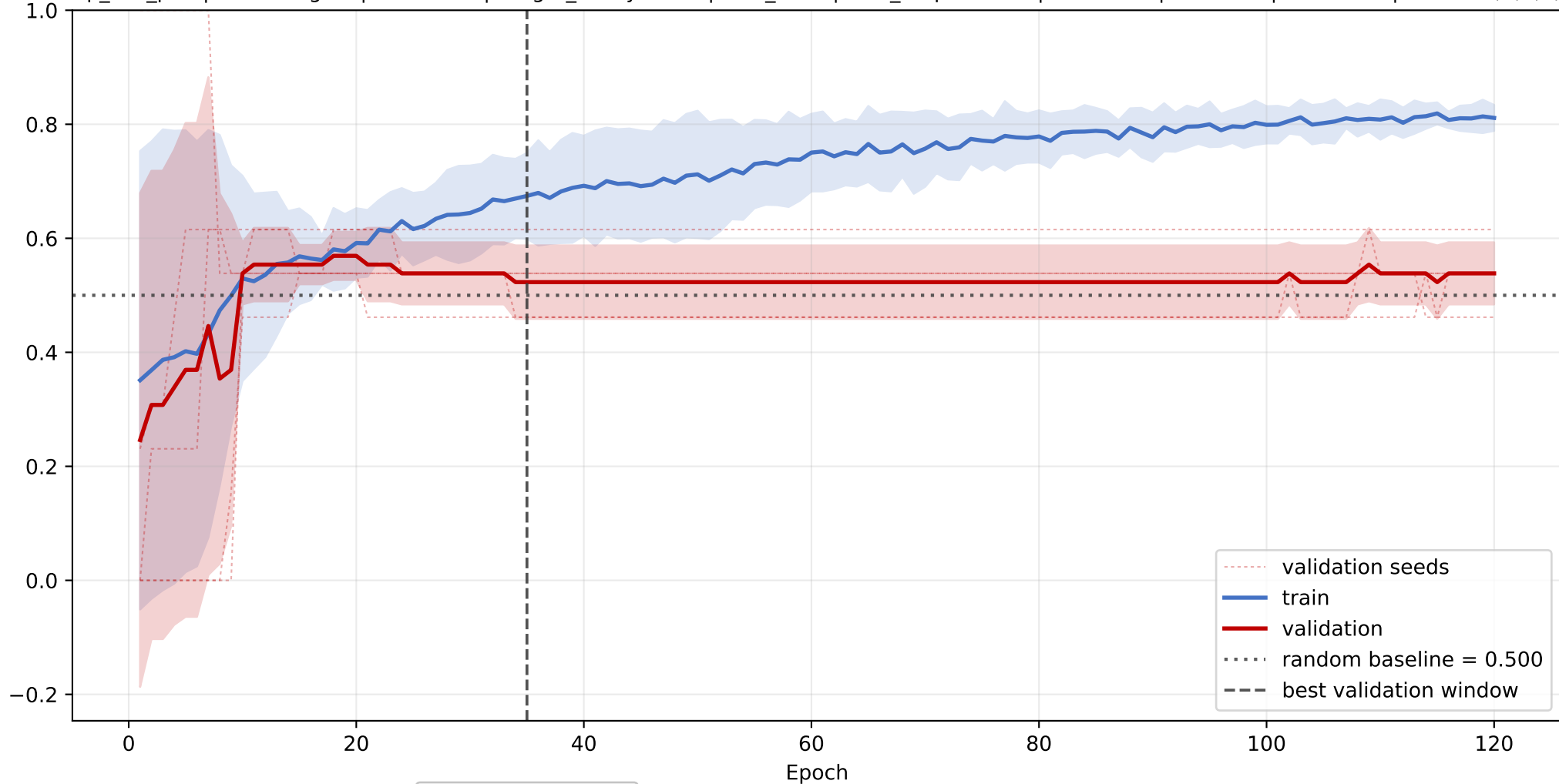
PA: mean sensitivity learning curve across seeds
