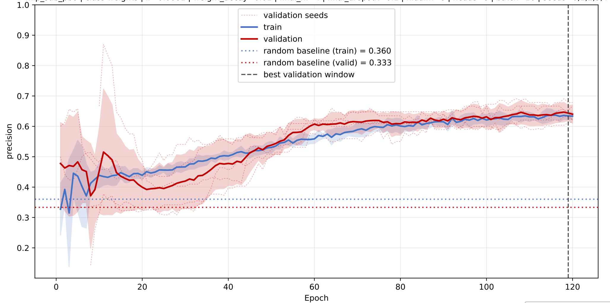
PE: mean precision learning curve across seeds
