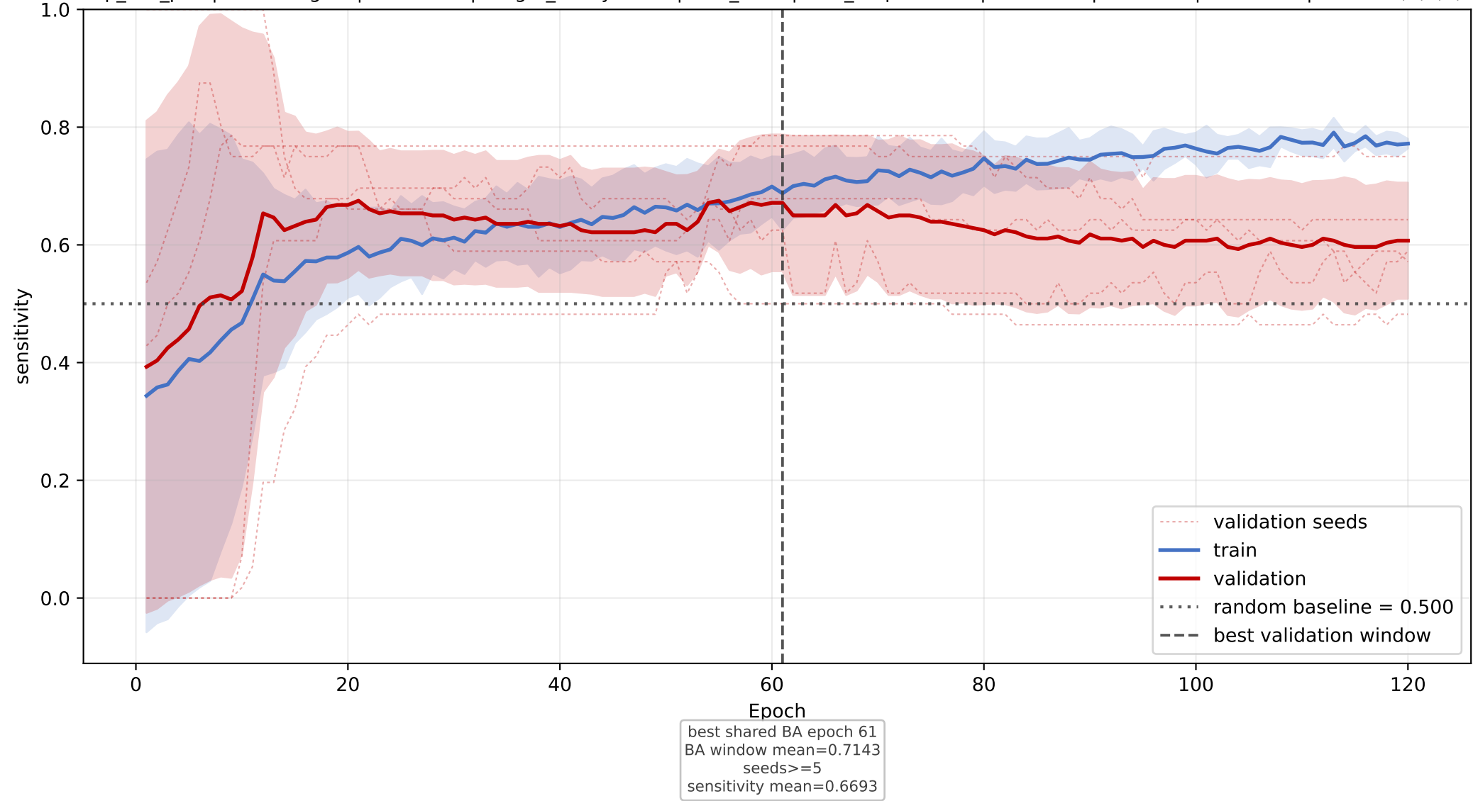
PG: mean sensitivity learning curve across seeds
