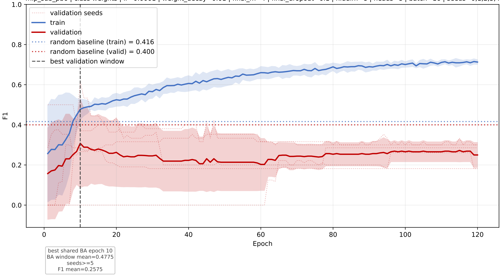
PS+PGP+DAG+TAG: mean F1 learning curve across seeds
