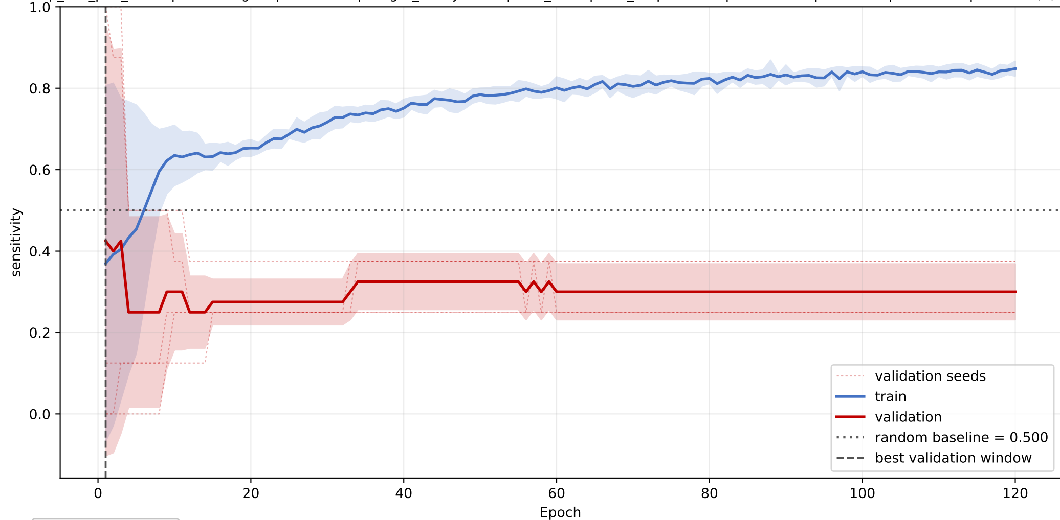
PS+PGP+DAG+TAG: mean sensitivity learning curve across seeds
