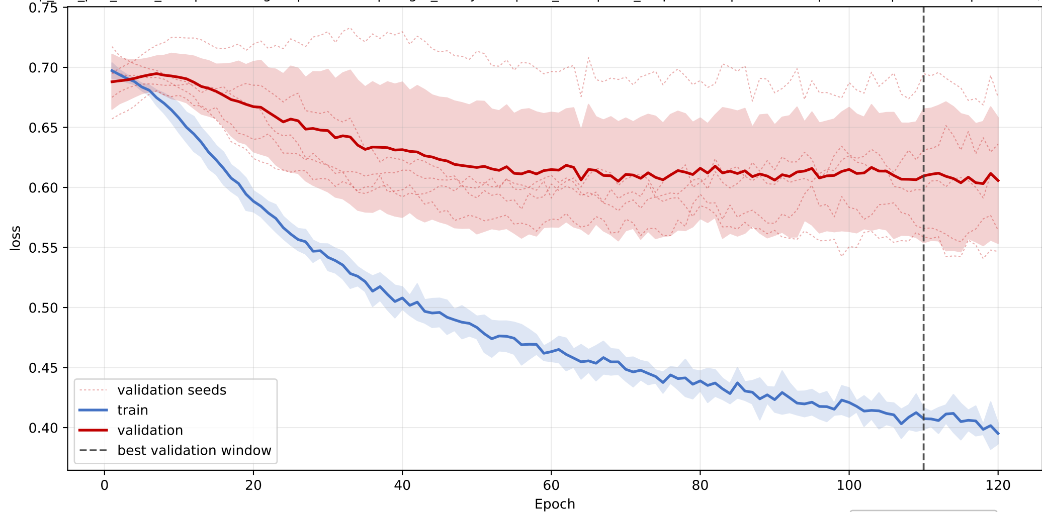
LPC+LPE+LPG: mean loss learning curve across seeds
