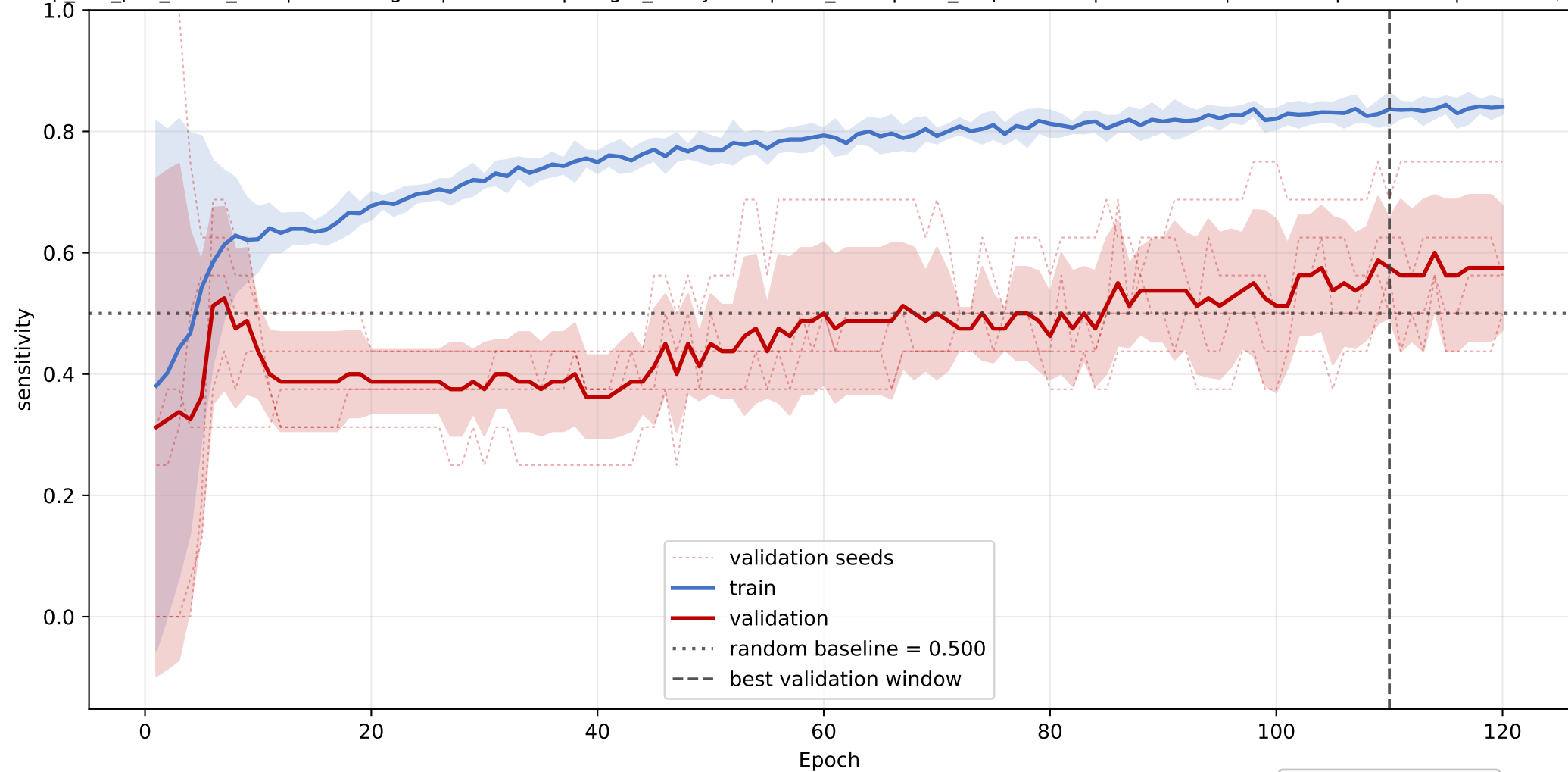
LPC+LPE+LPG: mean sensitivity learning curve across seeds
