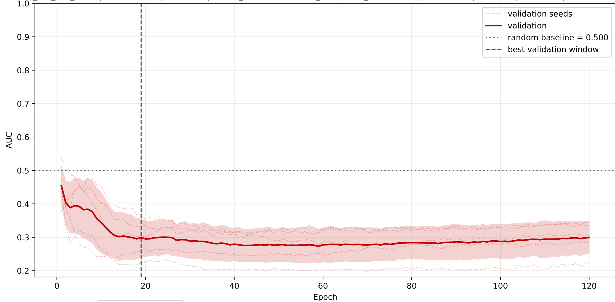
FA: mean AUC learning curve across seeds
