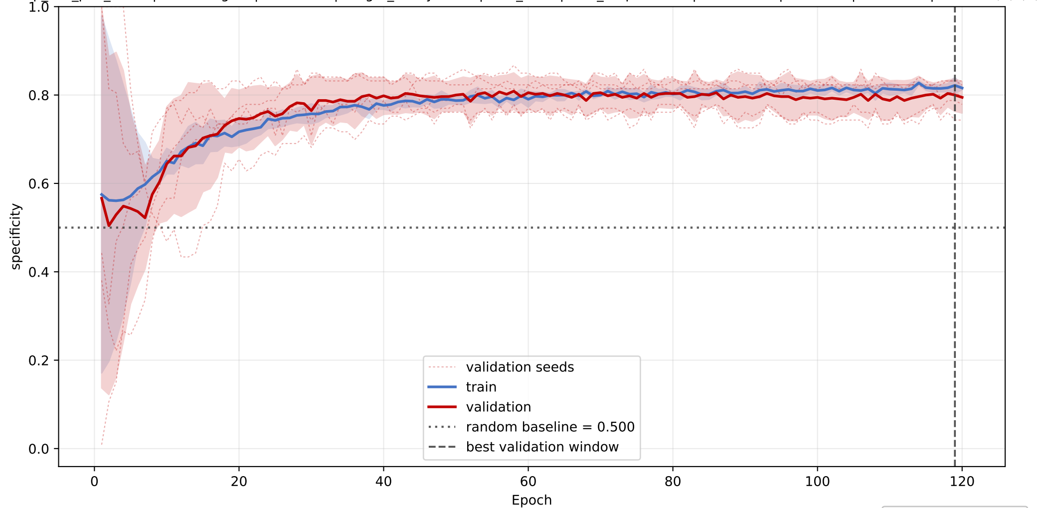
PG: mean specificity learning curve across seeds
