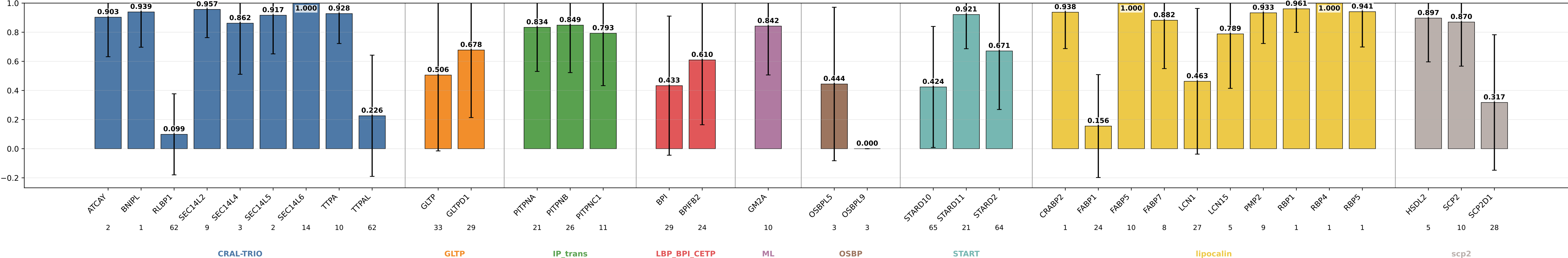
mlp_sub_pb6_hid32 specificity by subgroup mlp_sub_pb6_hid32 | class weights | lr=0.0001 | weight_decay=0.01 | final_m=4 | final_dropout=0.1 | hiddim=32 | heads=8 | batch=16 | ep=120 | seeds=0,1,2,3,4
