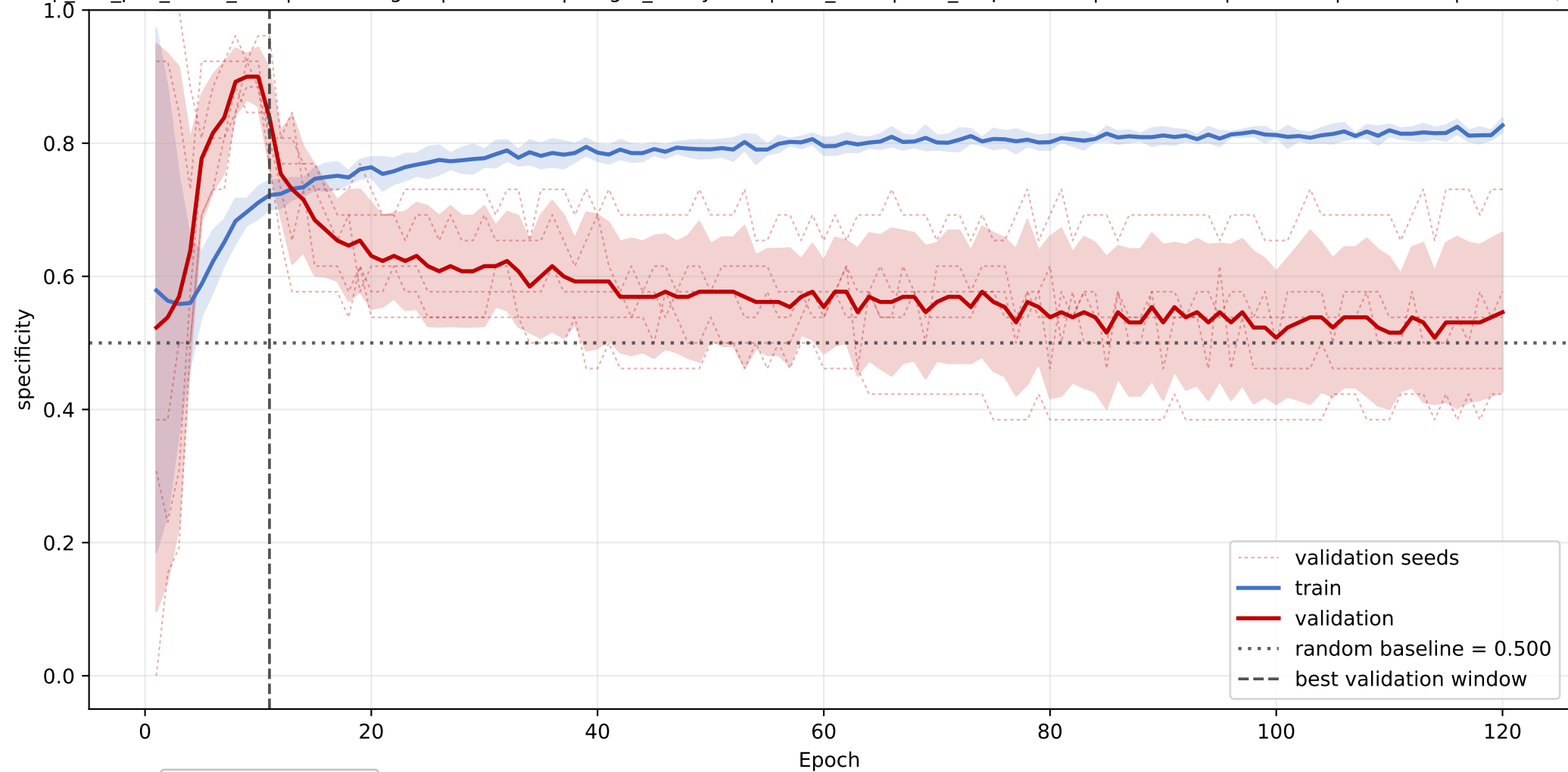
PA: mean specificity learning curve across seeds
