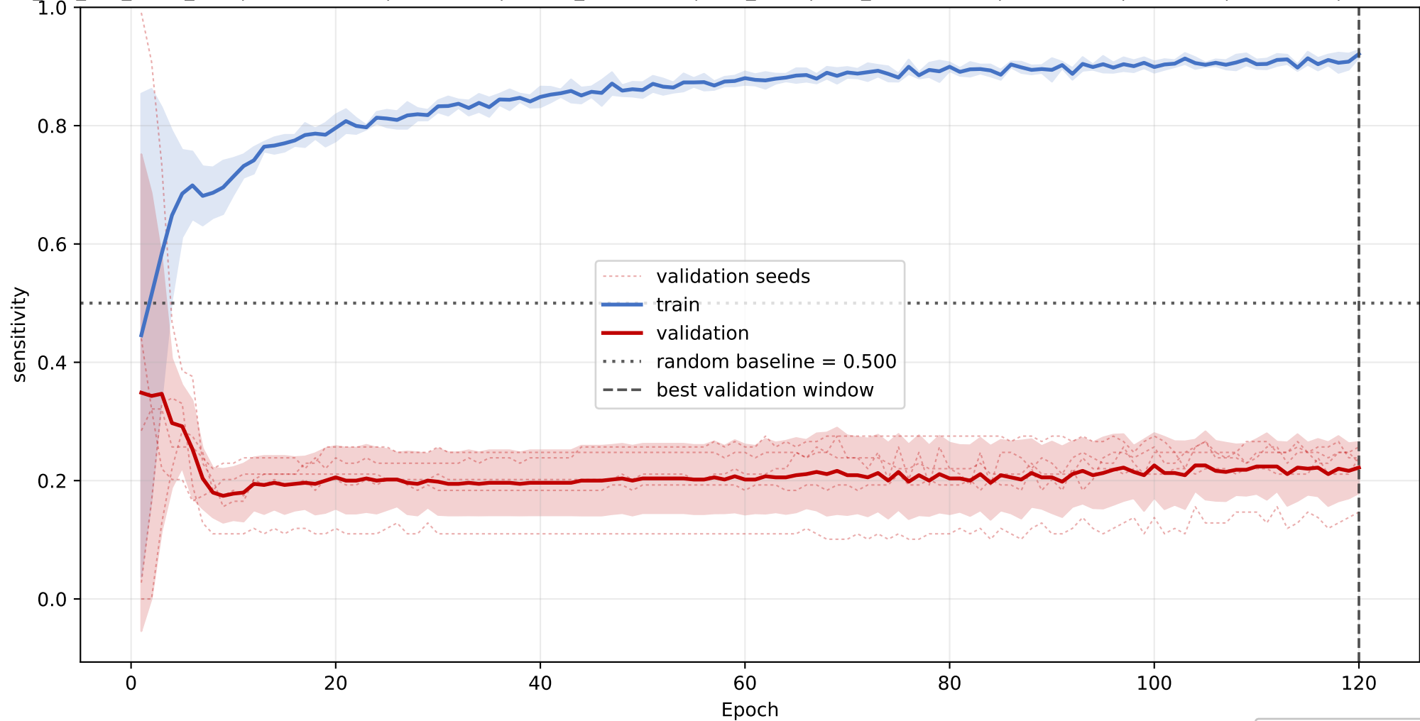
PC: mean sensitivity learning curve across seeds
