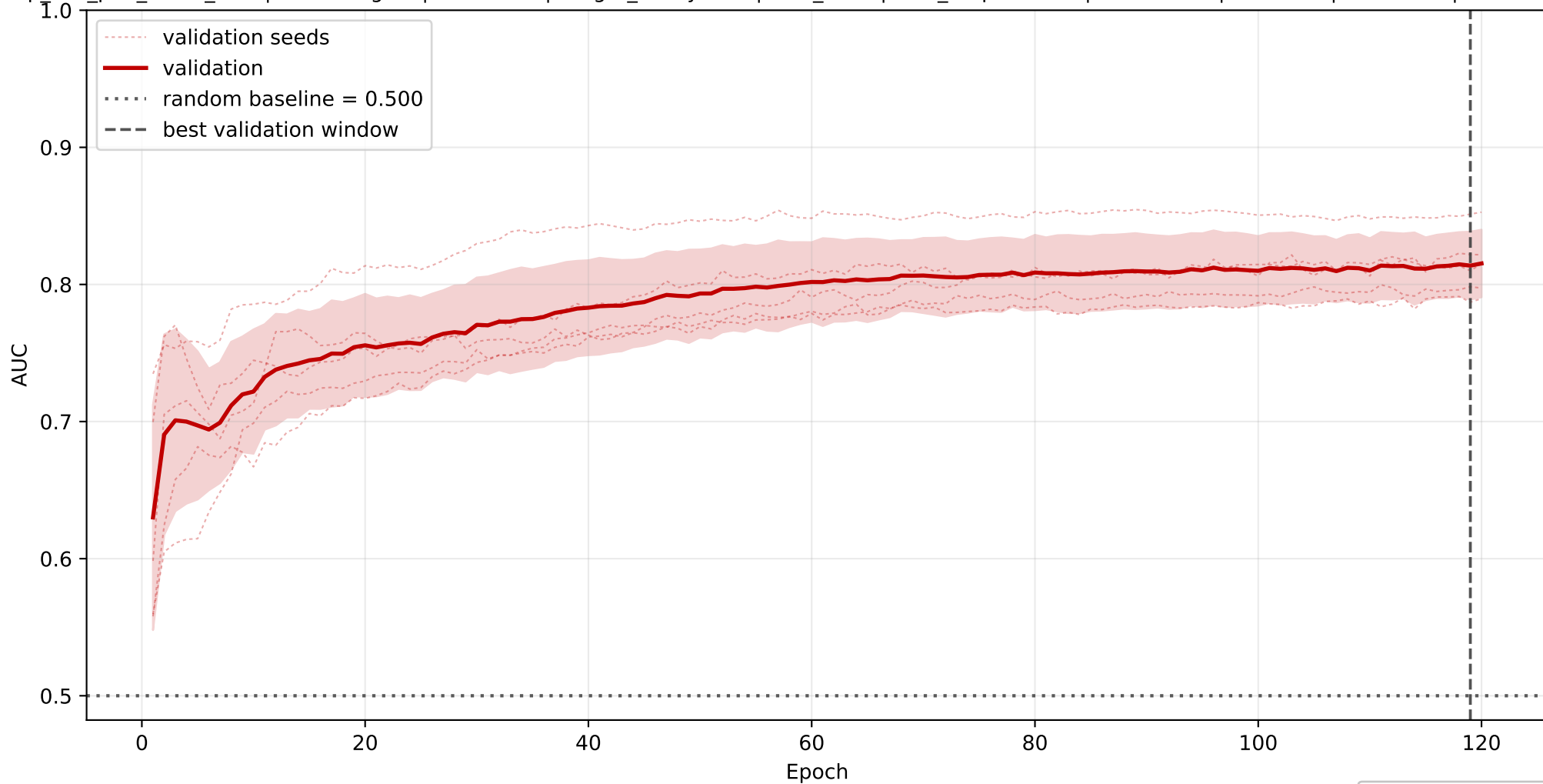
PG: mean AUC learning curve across seeds
