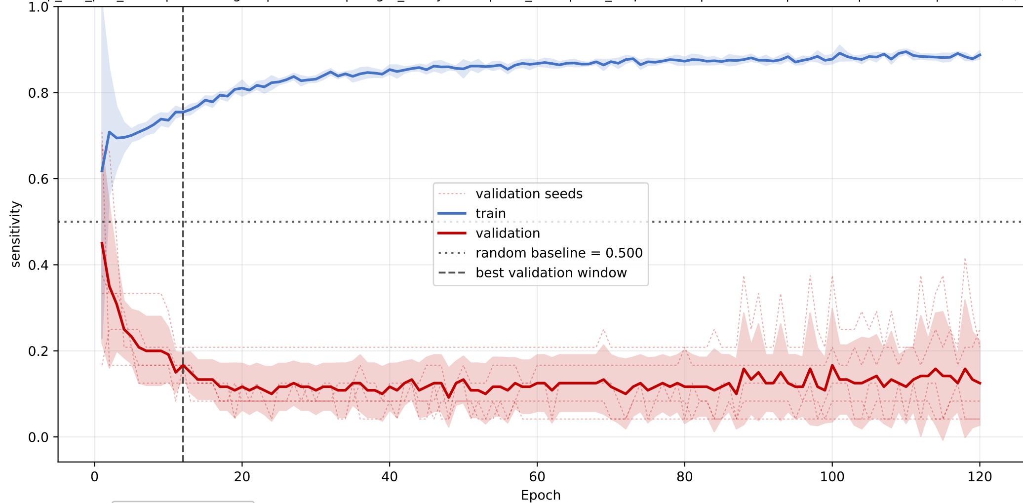
FA: mean sensitivity learning curve across seeds
