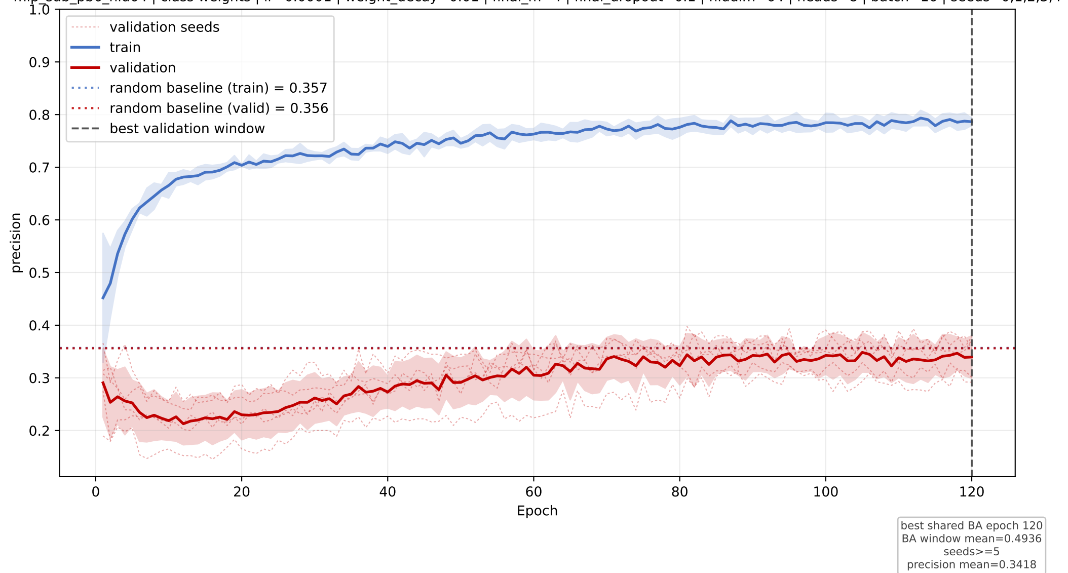
PC: mean precision learning curve across seeds
