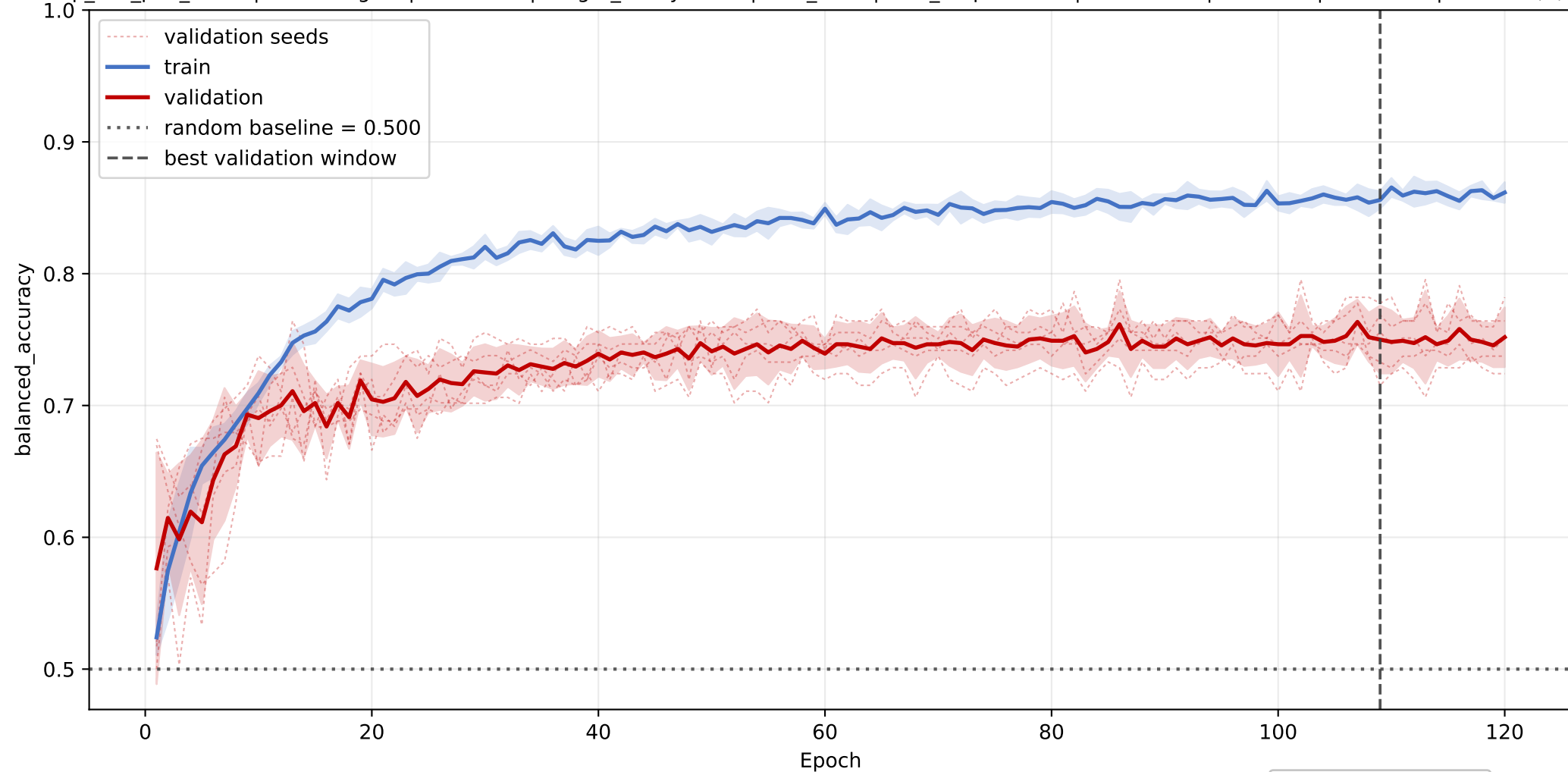
PG: mean balanced_accuracy learning curve across seeds
