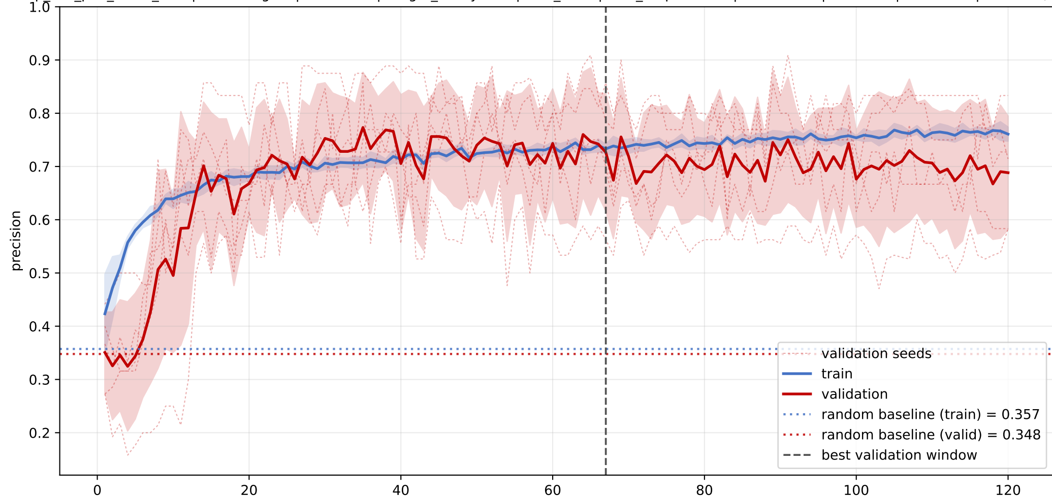
LPC+LPE+LPG: mean precision learning curve across seeds
