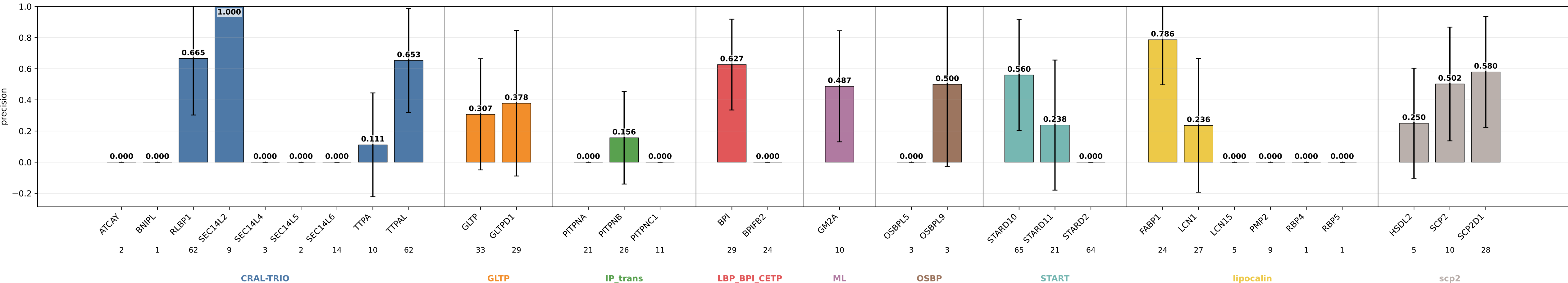
mlp_sub_pb6_hid64_wd0 precision by subgroup mlp_sub_pb6_hid64_wd0 | class weights | lr=0.0001 | weight_decay=0.0 | final_m=4 | final_dropout=0.1 | hiddim=64 | heads=8 | batch=16 | ep=120 | seeds=0,1,2,3,4
