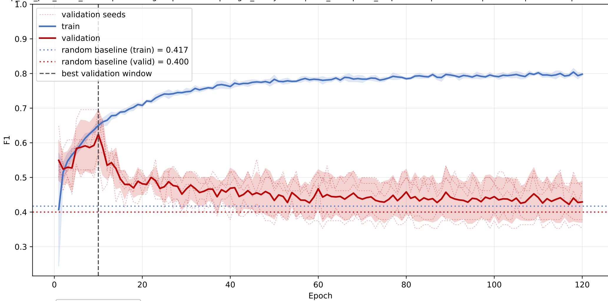
PA: mean F1 learning curve across seeds
