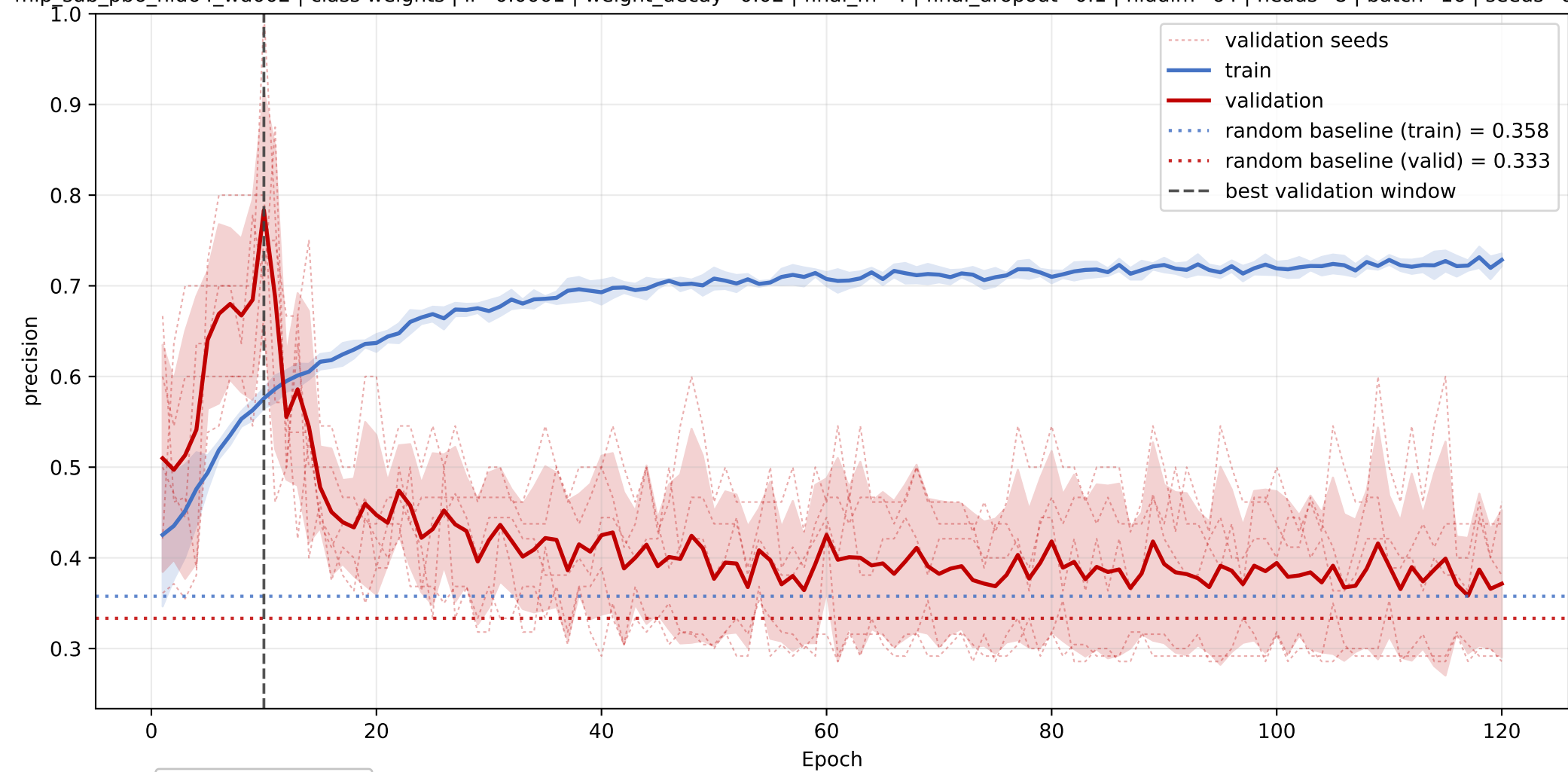
PA: mean precision learning curve across seeds
