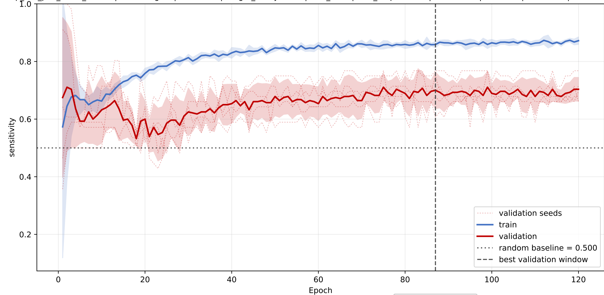
PG: mean sensitivity learning curve across seeds
